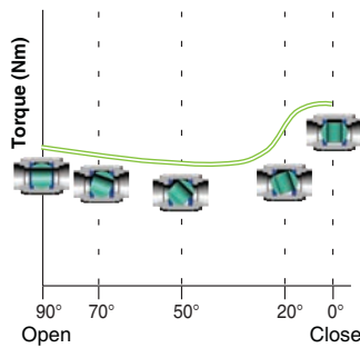
Ball valve
