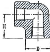
90° ELBOW
