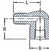
90° STREET ELBOW
